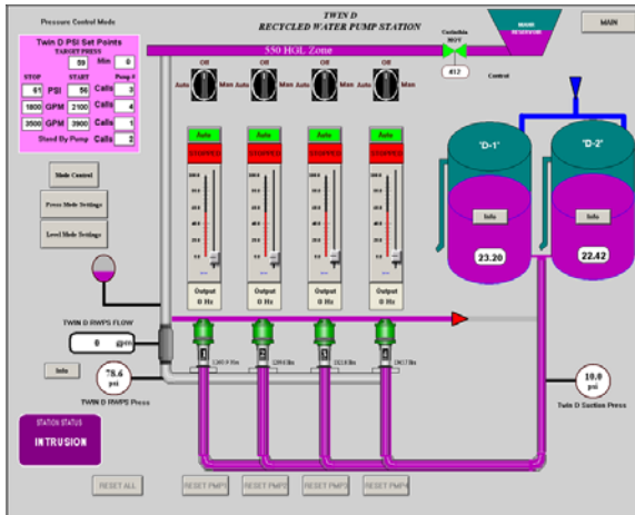
Pump station status is monitored via a WonderWare Intouch HMI.
