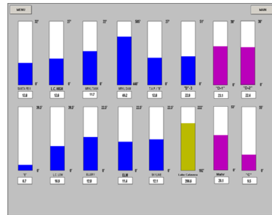
HMI screens display the water levels of tanks, lakes, and reservoirs that supply the city.
